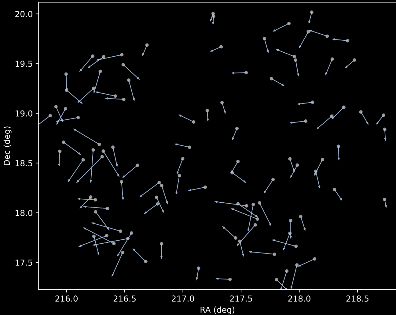
APOGEE DR17 Cluster 1 Proper Motion Vectors (n=102)
