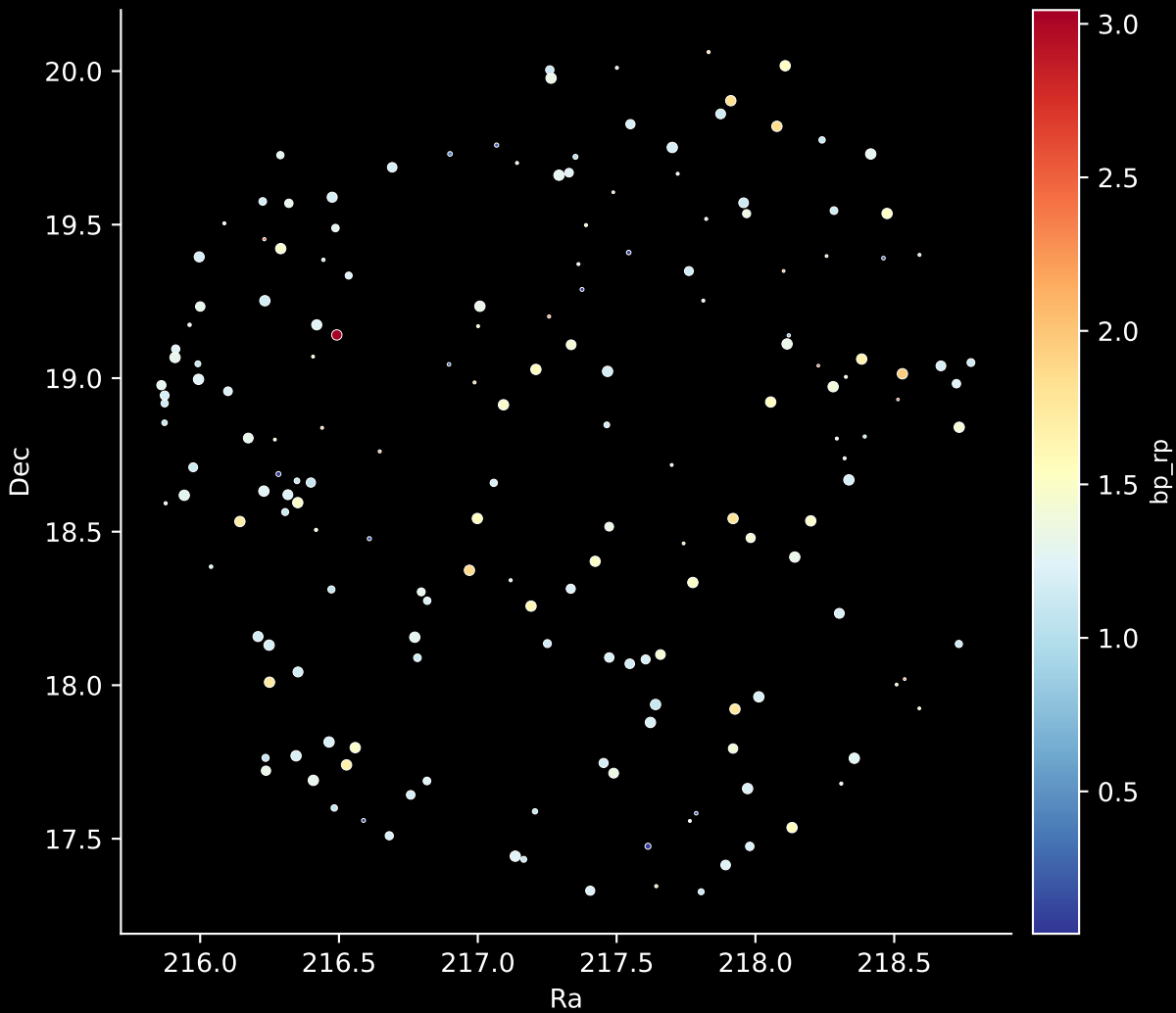
APOGEE DR17 Field: [202+21_MGA] Stars: 175
