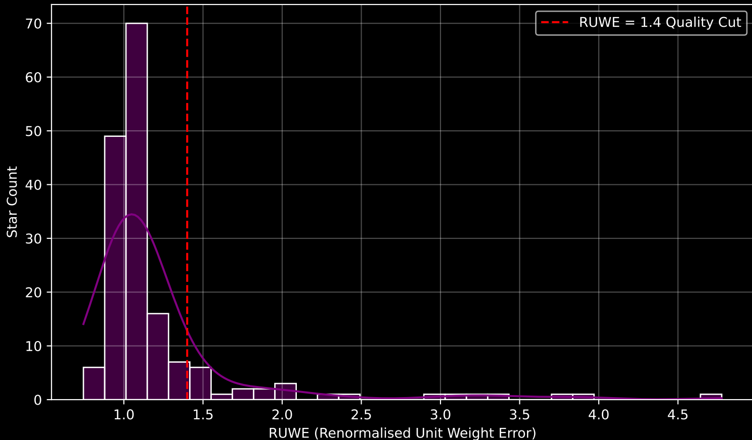
GAPOGEE DR17 Field [202+21_MGA] RUWE Distribution (n= 171)
