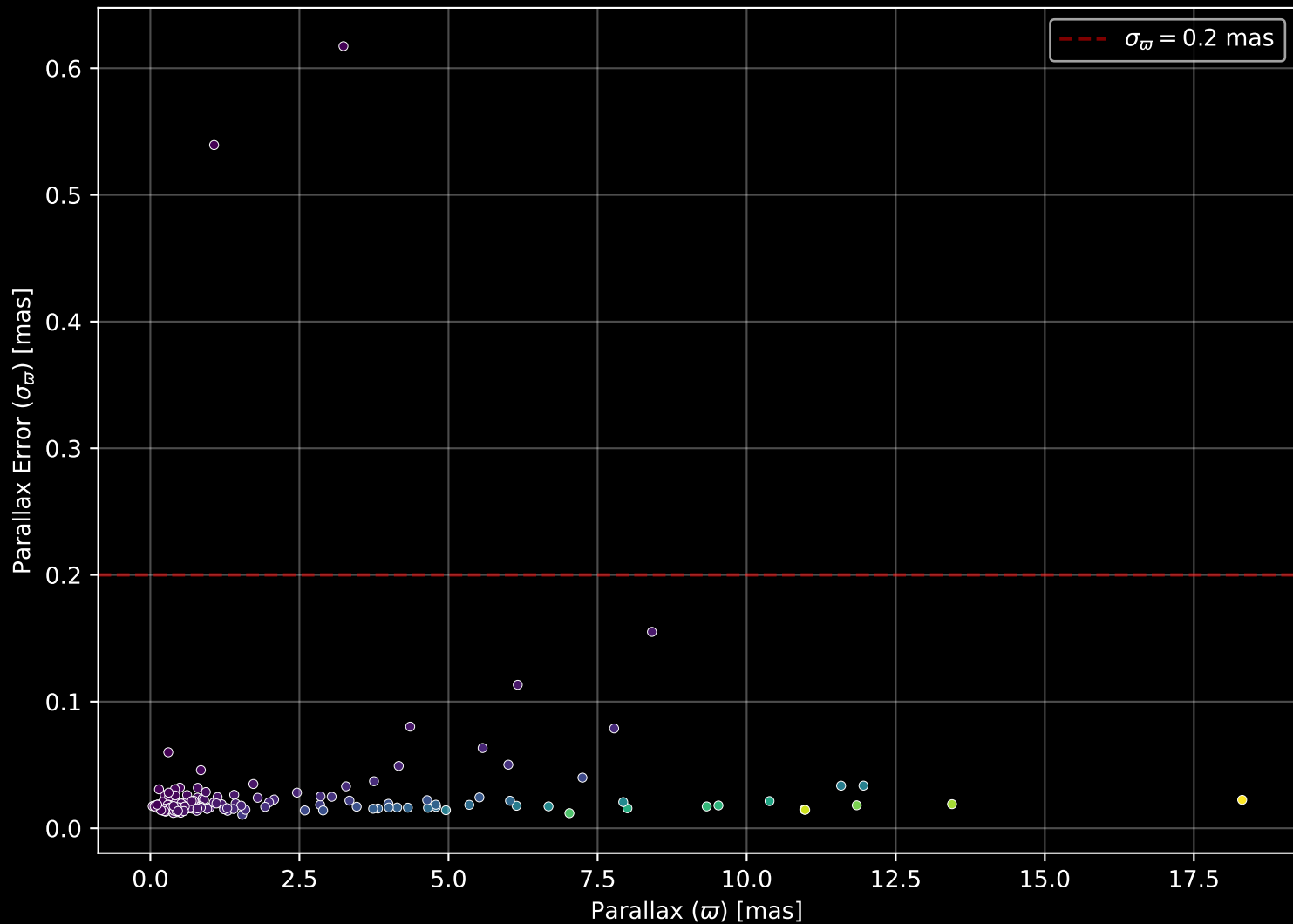
APOGEE DR17 Field: [202+21_MGA] Parallax Quality (n= 175)
