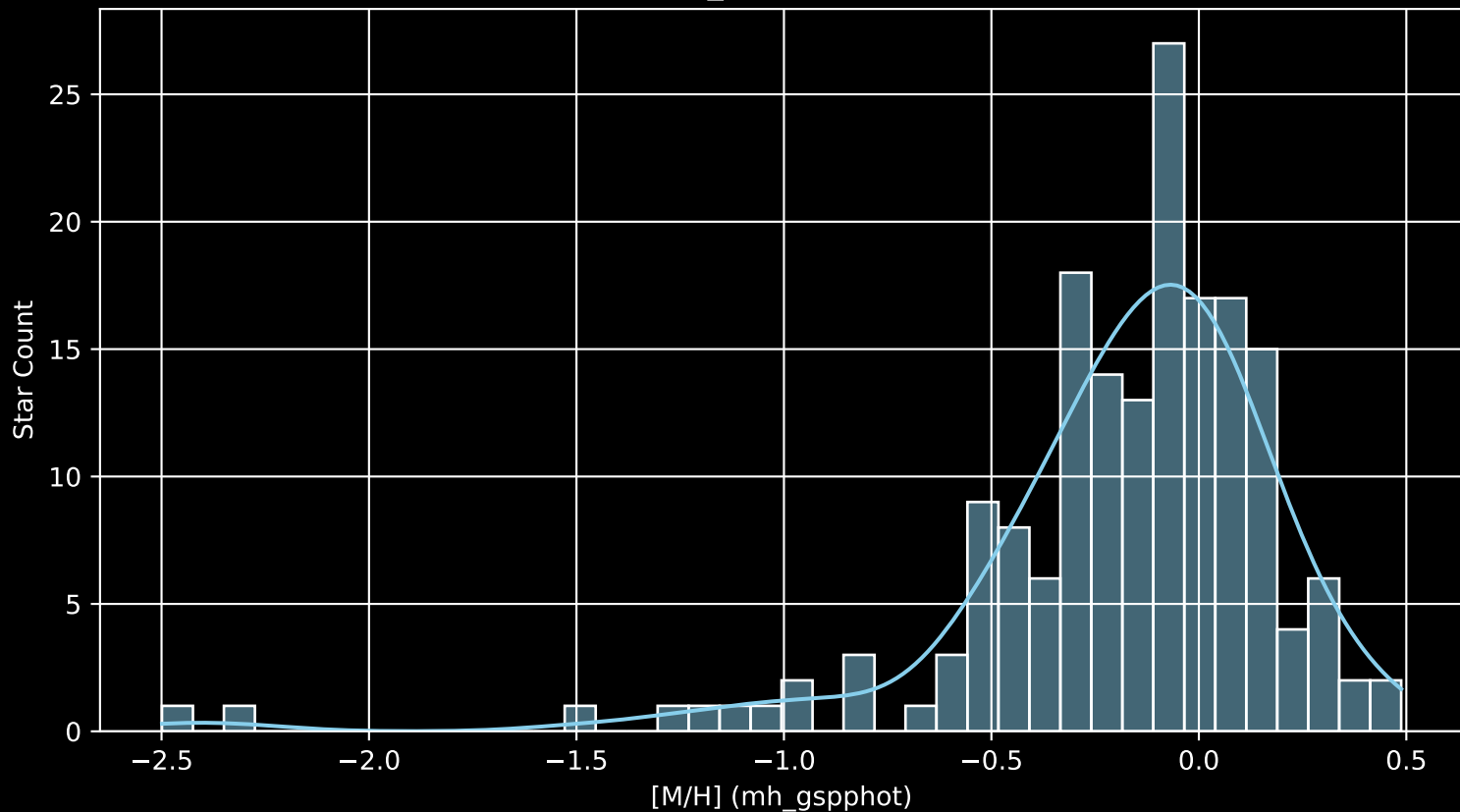
APOGEE DR17 Field: [202+21_MGA [M/H] (mh_gspphot) (n= 174)
