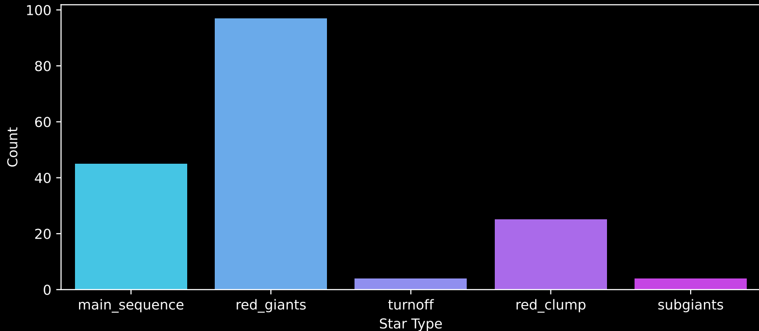
APOGEE DR17 Field: [202+21_MGA] Count plot of Star Type
