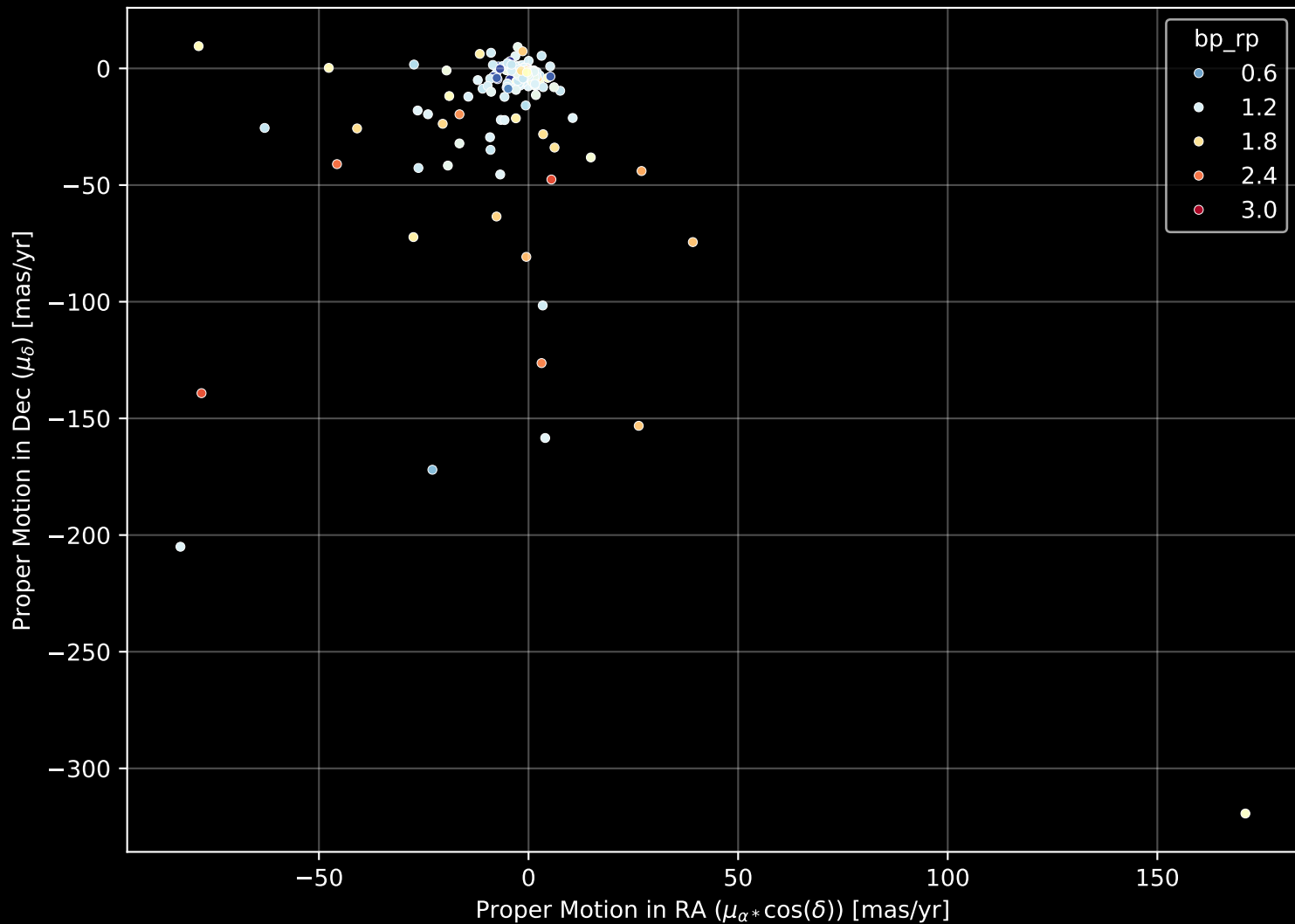
APOGEE DR17 Field: [202+21_MGA] Proper Motion Diagram (n= 175)
