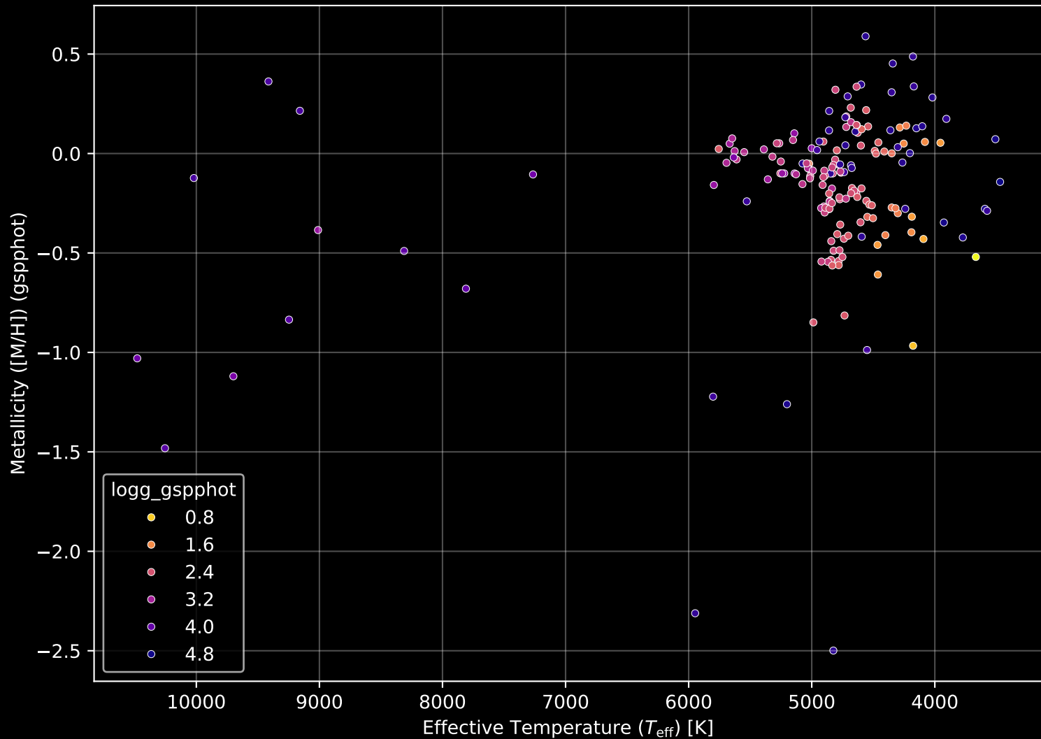
APOGEE DR17 Field: [202+21_MGA] Stellar Population Parameters (n= 175)
